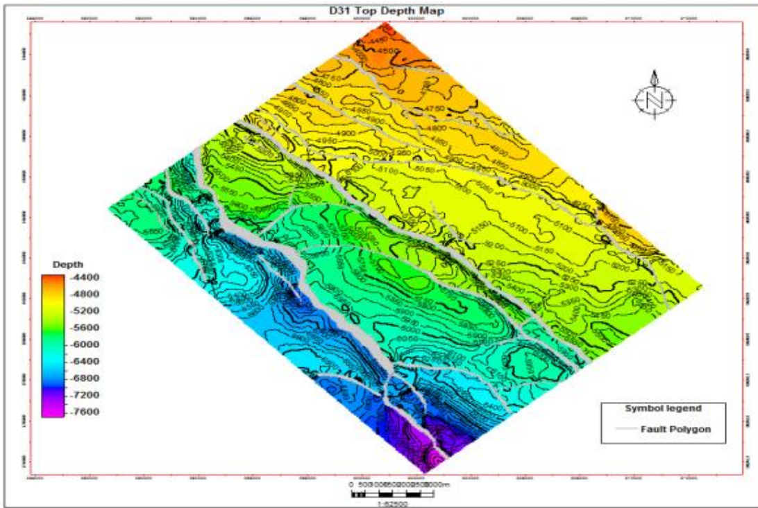
Fig. 13. Depth structure map of horizon D31
