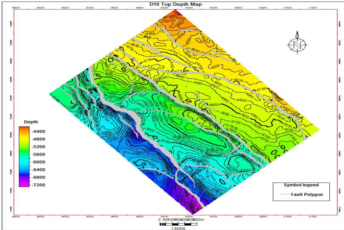
Fig. 12. Depth structure map of horizon D10
