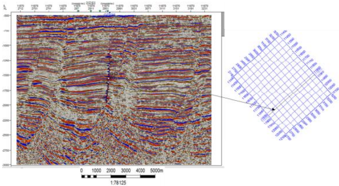
Fig. 8. Synthetic seismogram of Otu36 and the mapped well tops
