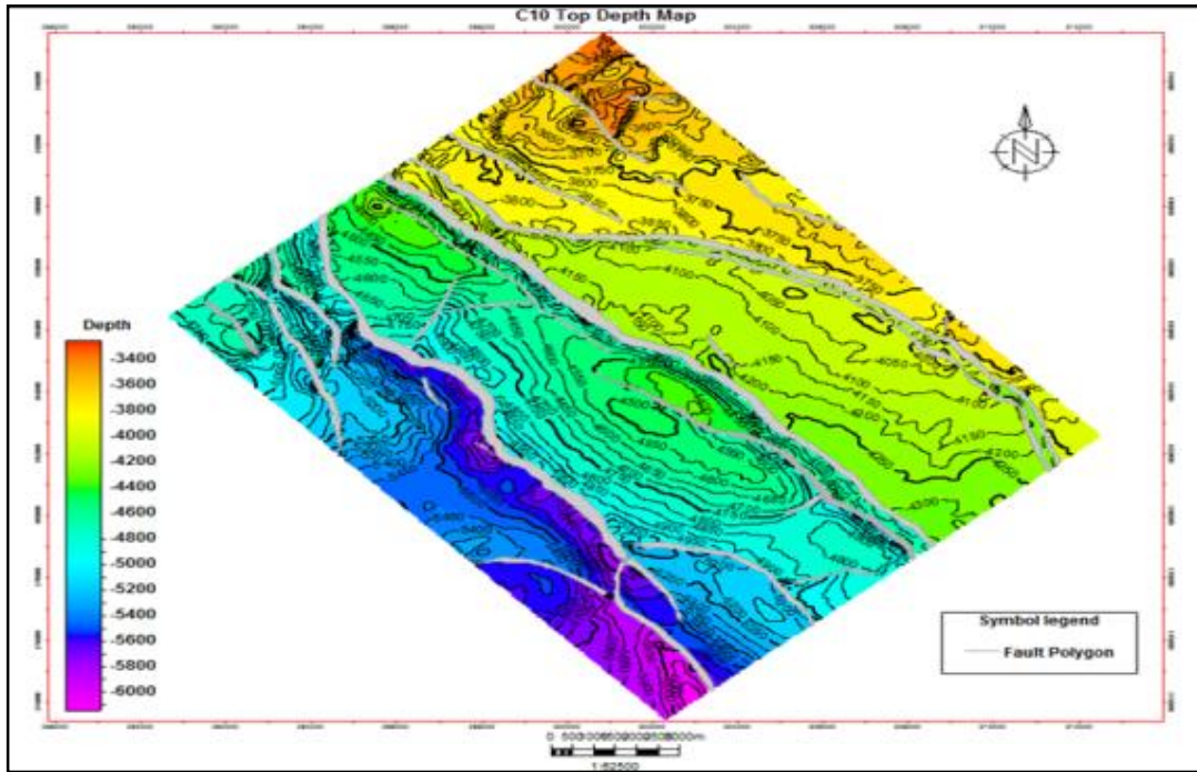
Fig. 11. Depth structure map of horizon C10
