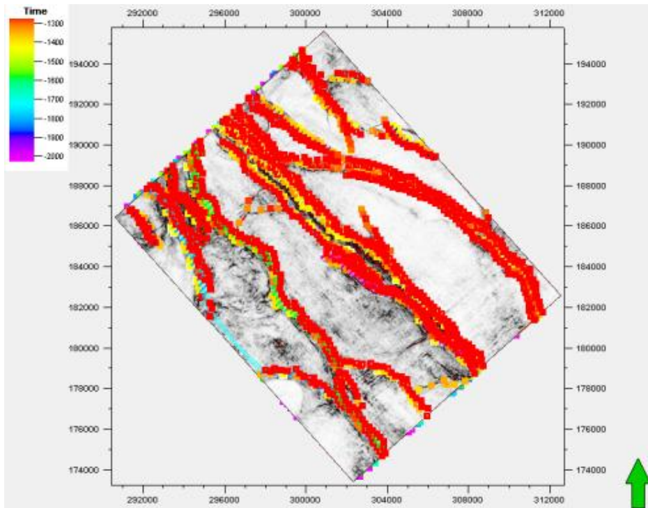
Fig. 10. Variance time slice with fault sticks
