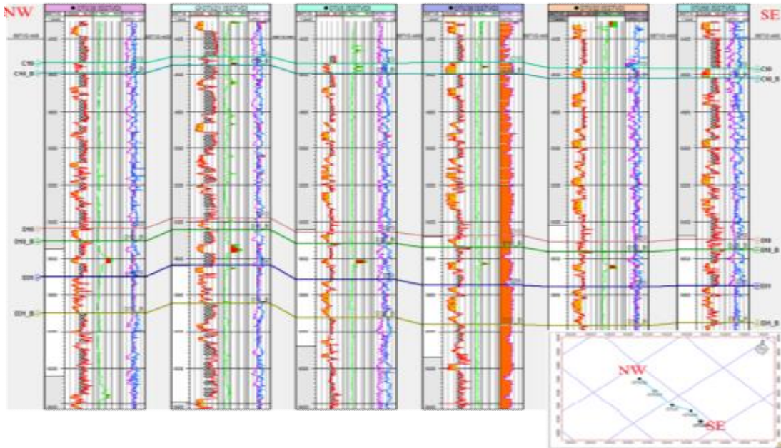
Fig. 7a. Well correlation panel of Otu field
