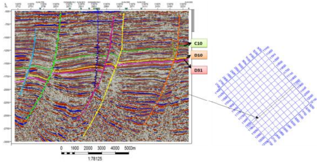
Fig. 9. Seismic Inline showing fault sticks and horizons interpreted
