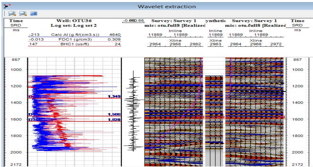
Fig. 6. Sonic calibration Otu36
