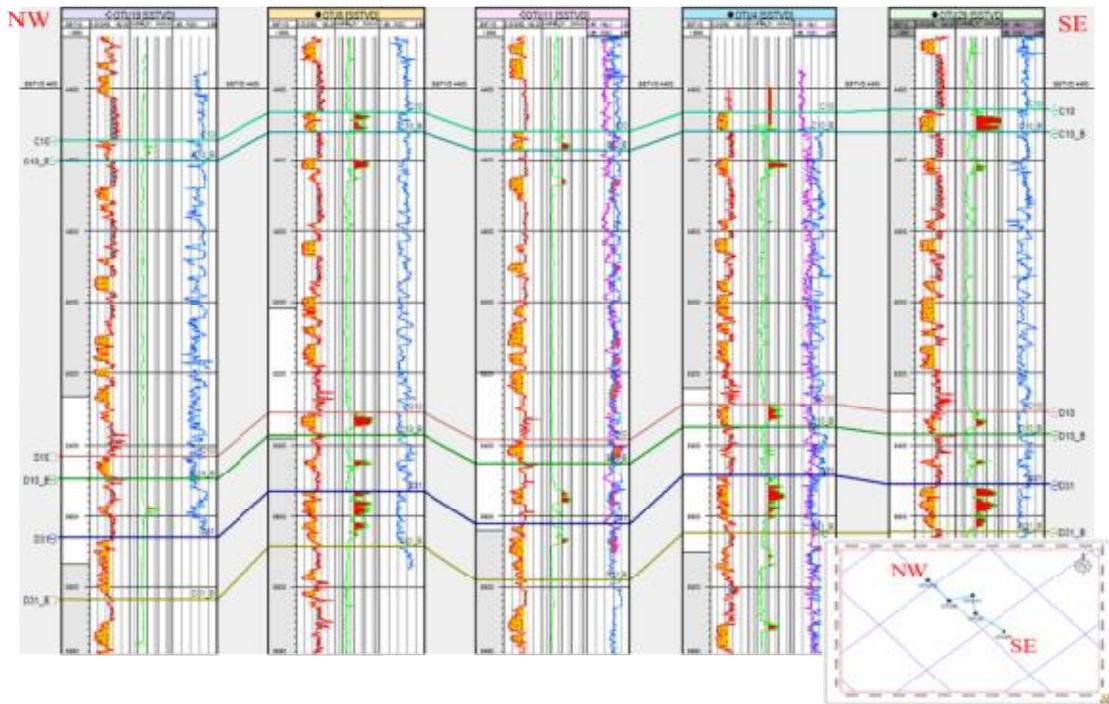
Fig. 7b. Well correlation panel of Otu Field contd
