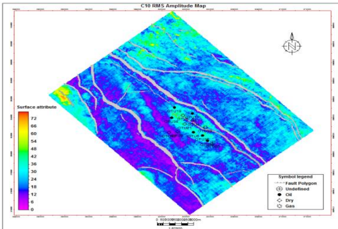
Fig. 14. RMS amplitude for horizon C10
