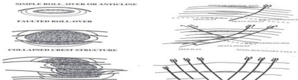
Fig. 4. Conventional trapping configuration in the Niger Delta (Modified from [17])
