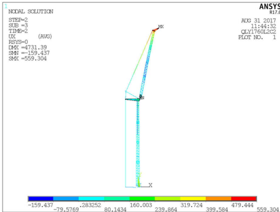
Fig. 4. Cloud image of tower crane deformation result
