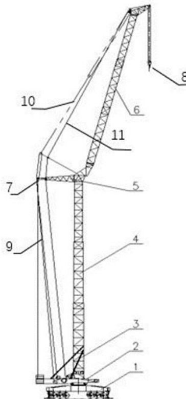
Fig. 1. Machine structure drawing
