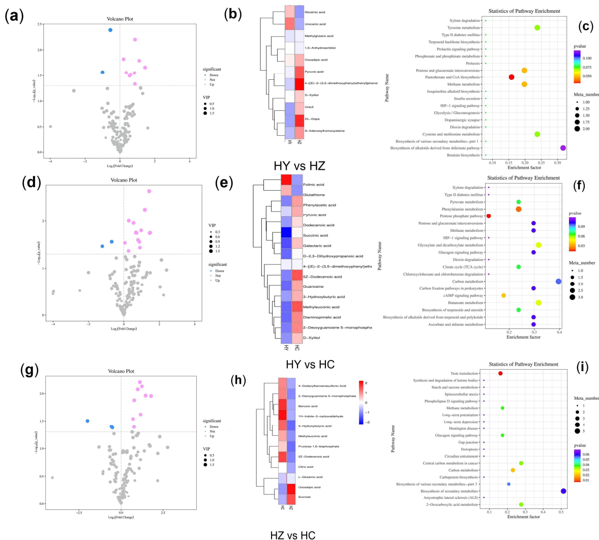
Figure 2. A comparative analysis of the different metabolite types in the different developmental stages of Caoyuanheimo-1 ( Agaricus sp.). HY represents the primordium period of Caoyuanheimo-1, HZ represents the young fruiting period of Caoyuanheimo-1, and HC represents the ripe fruiting period of Caoyuanheimo-1. Volcano plots show the differentially accumulated metabolites between the HY vs. HZ (a), HY vs. HC (d), and HZ vs. HC (g) groups. Each point in the volcano map represents a metabolite; the X axis represents the logarithm of the fold change of a certain metabolite in the two samples; and the Y axis represents the logarithm of the p -value. The blue dots represent downregulated differentially accumulated metabolites; the pink dots represent upregulated differentially accumulated metabolites; and gray represents detected but not significantly differentially accumulated metabolites. The size of the dots represents different VIP values. Heatmaps visualization shows the differential metabolites accumulated between the HY vs. HZ (b), HY vs. HC (e), and HZ vs. HC (h) groups. The relative accumulation levels of individual samples are shown; the transition from red to blue represents the level of metabolite accumulation. The differentially accumulated metabolite enrichment analysis of the different development stages are shown as bubble charts of the KEGG enrichment analyses by the HY vs. HZ (c), HY vs. HC (f), and HZ vs. HC (i) groups.
