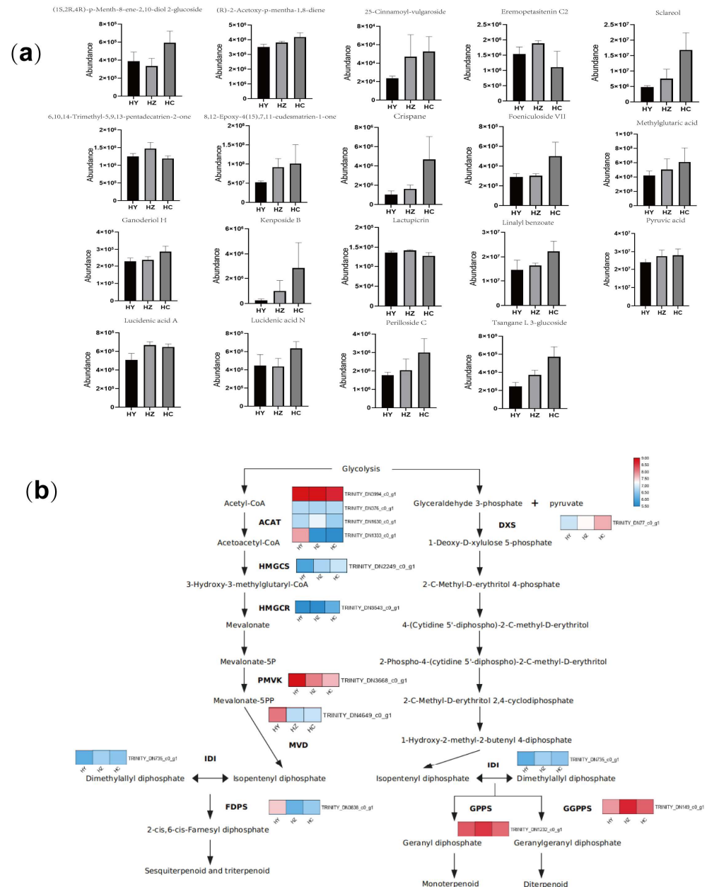
Figure 5. An analysis of the key genes in the synthesis pathway of terpenoids and the content of terpenoids during growth and development. (a) The bar chart represents the content of terpenoid metabolites and substrates at three different developmental stages; HY represents the primordium period of Caoyuanheimo-1; HZ represents the young fruiting period of Caoyuanheimo-1; and HC represents the ripe fruiting period of Caoyuanheimo-1. (b) The heatmap represents the expression levels of key genes in the terpenoid biosynthesis pathway in the HY, HZ, and HC groups. The scale of the heatmap represents the FPKM of genes.
