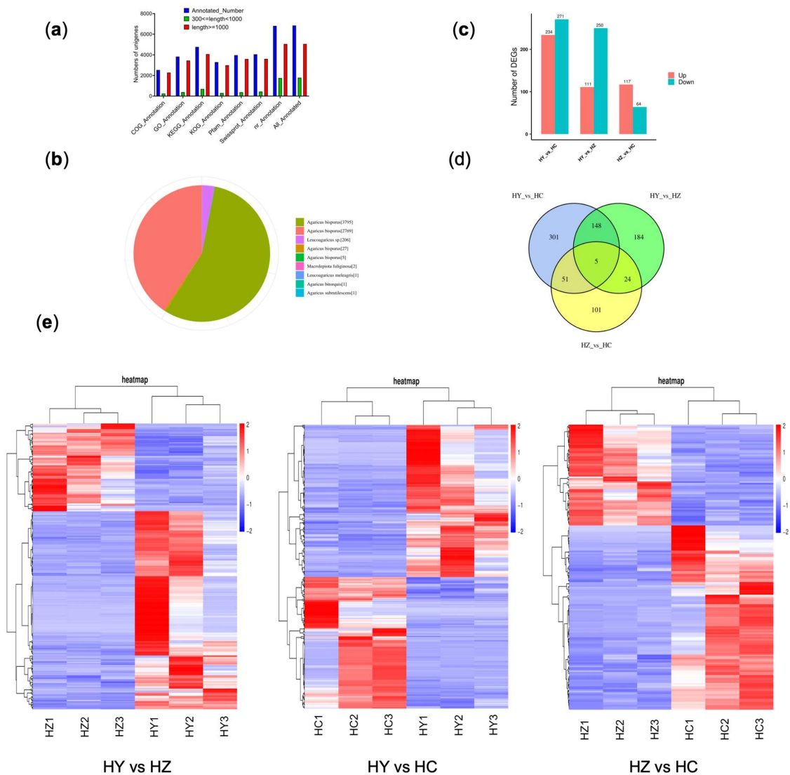
Figure 3. A differential gene analysis between the different development stages: HY represents the primordium period of Caoyuanheimo-1 ; HZ represents the young fruiting period of Caoyuanheimo-1 ; and HC represents the ripe fruiting period of Caoyuanheimo-1 . (a) Functional annotation numbers of the unigenes in the COG, GO, KEGG, KOG, Pfam, Swissprot, and NR databases. (b) An annotated species distribution in the NR database. (c) A statistical analysis of the number of upregulated and downregulated DEGs in the HY vs. HC, HY vs. HZ, and HZ vs. HC groups, respectively. (d) A Venn diagram showing the shared and unique genes among the HY vs. HZ, HY vs. HC, and HZ vs. HC groups. The numbers represent the number of genes that were unique or shared. (e) The heatmap is linked by a dendrogram representing clustering of the transcriptomic data. The color code is as follows: red indicates upregulated transcripts; blue indicates downregulated transcripts; and white indicates unchanged transcripts. The color scale of the heatmap ranges from blue (−2.0) to red (2.0) in the natural logarithmic scale.
