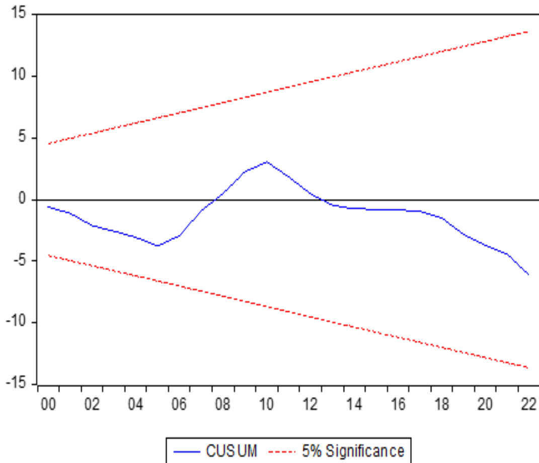
Fig. 1. CUSUM test for autoregressive distributed lag model stability
