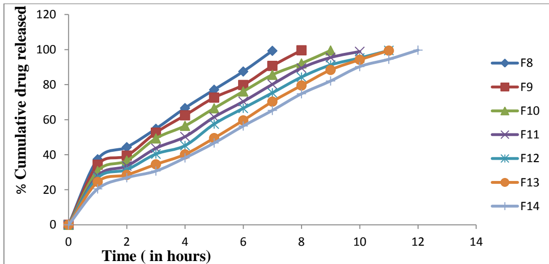
Fig. 4. In-vitro dissolution profile of F8-F14 formulation
