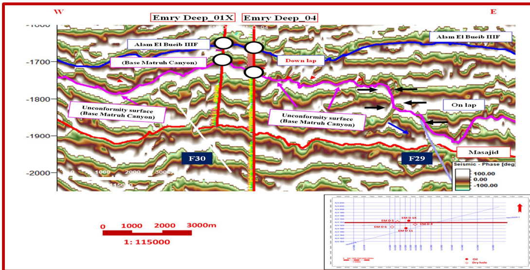
Figure 5. Instantaneous phase for XLN 1920, with the stratigraphic terminations.
