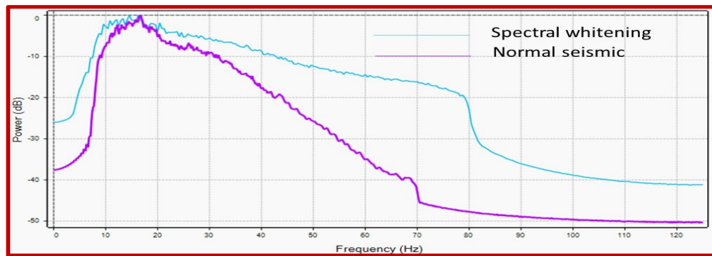
Figure 10. Frequency spectrum for normal seismic and spectral whitening at Xline 1920.
