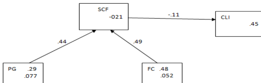
Fig. 1. Basic SEM PLS algorithms for a socio-cultural model of child labour
