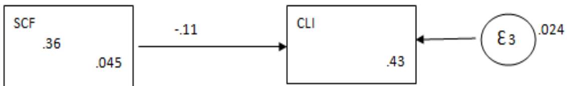
Fig. 2. SEM PLS Optimal inner structural sociocultural model Source: Author (2023)
