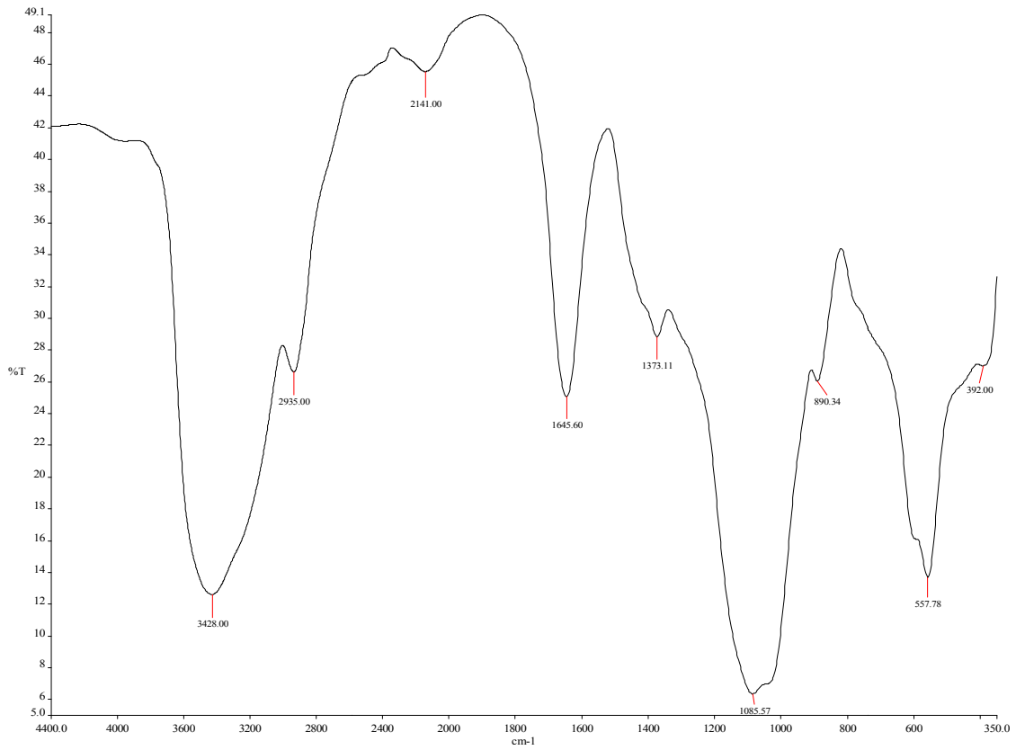
Fig. 11. FTIR Spectrum of produced PHA from isolate L. casei WWD3
