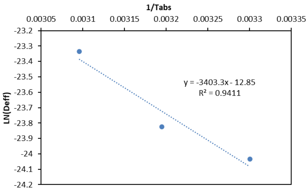
Fig. 5. \text{Ln } D_{eff} vs 1/T_{abs} of drumstick leaf drying
