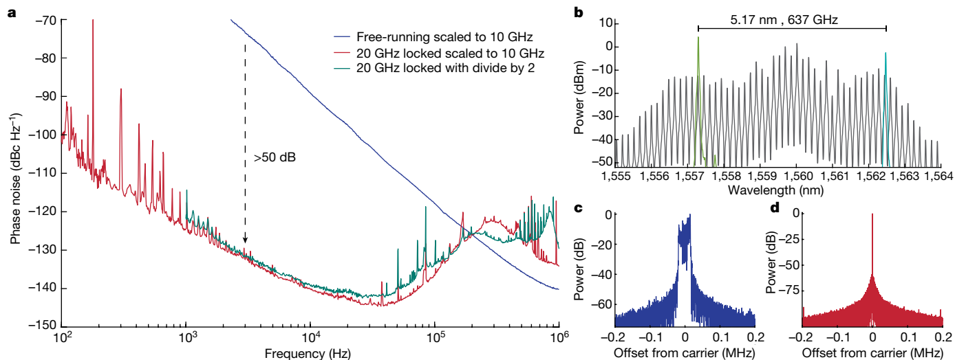
Fig. 3 | Microcomb characterization. a , Single side-band phase noise scaled to 10 GHz of free-running 20 GHz microcomb (blue), locked 20 GHz microwave (red) and locked 20 GHz microwave after regenerative frequency division by
