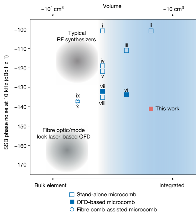
Fig. 4 | Phase noise comparison of microwave generation based on microcombs. The platforms are all scaled to 10 GHz carrier and categorized based on the integration capability of the microcomb generator and the reference laser source, excluding the interconnecting optical/electrical parts. Filled (blank) squares are based on the OFD (stand-alone microcomb) approach: (i) 22 GHz silica microcomb 50 ; (ii) 5 GHz Si 3 N 4 microcomb 14 ; (iii) 10.8 GHz Si 3 N 4 microcomb 32 ; (iv) 22 GHz microcomb 31 ; (v) MgF 2 microcomb 32 ; (vi) 100 GHz Si 3 N 4 microcomb 33 ; (vii) 22 GHz fibre-stabilized SiO 2 microcomb 21 ; (viii) MgF 2 microcomb 53 ; (ix) 14 GHz MgF 2 microcomb pumped by an ultrastable laser 30 ; and (x) 14 GHz microcomb-based transfer oscillator 31 . SSB, Single side band.
