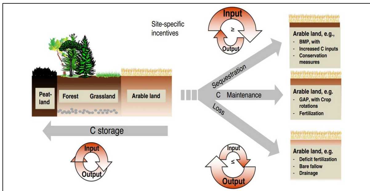
Fig. 2. The loss of C after conversion of native ecosystems i.e. peat land, forest, and grassland to arable land [2]
