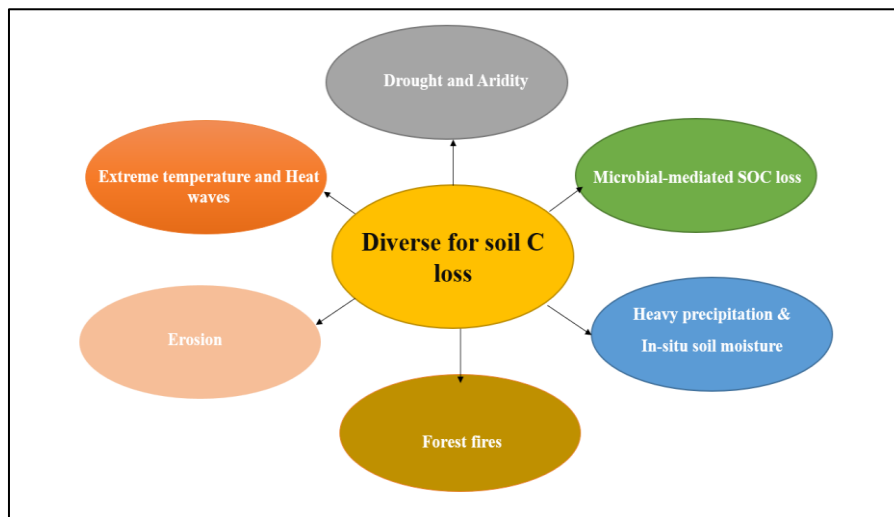
Fig. 1. Different divers for climate-induced soil carbon loss
