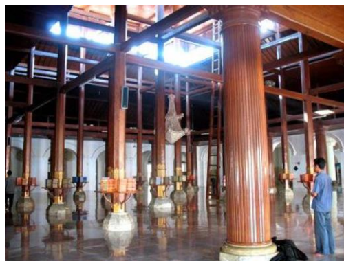
Fig. 3 Wooden construction in the main hall of the Ampel Mosque
