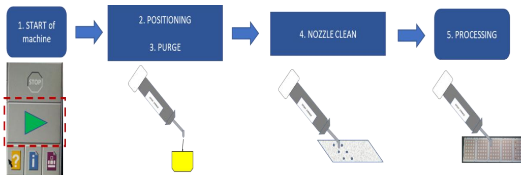
Fig. 8. Sequence of auto purge and nozzle cleaning
