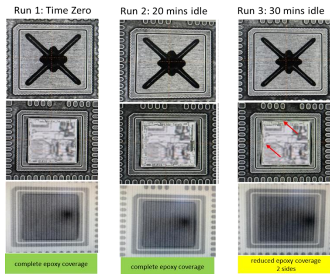
Fig. 5. Evaluation of idle time Runs 1-3
