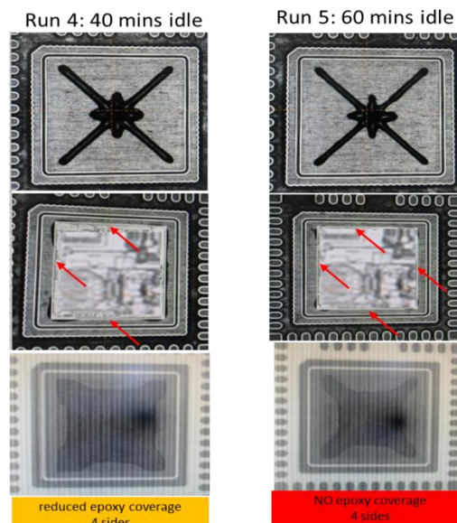
Fig. 6. (Cont.) Evaluation of idle time Runs 4-5
