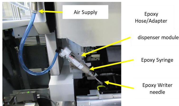
Fig. 3. Epoxy writer module of Die attach machine
