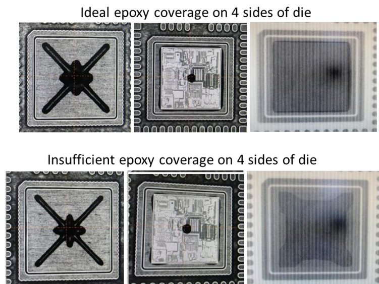
Fig. 4. Ideal and insufficient epoxy coverage shown on four sides of die
