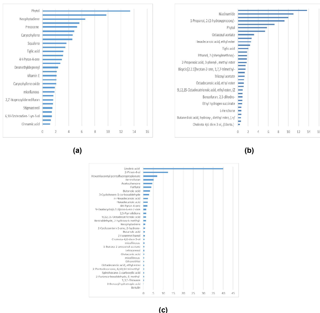
Fig. 3. Peak area percentage of compounds extracted from Etilingera elatior at different dosage of biochar; (a) 0% biochar, (b) 5% biochar and (c) 20% biochar
