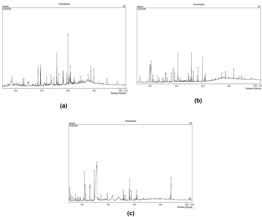
Fig. 2. Chromatogram of phytochemical from Etlingera elatior at different dosage of biochar; (a) 0% biochar, (b) 5% biochar and (c) 20% biochar
